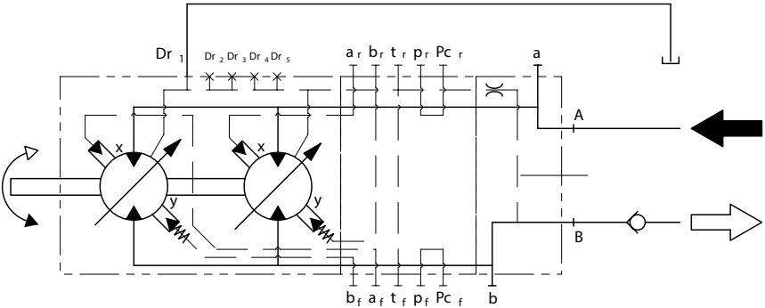
Circuit for case flushing, integrated supply, uni-directional. Contact KPM UK for this option.
