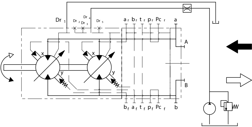
Circuit for case flushing, external supply, bi-directional
