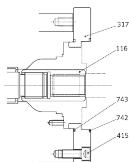
SAE "C" &amp; "C4" T/D Kit
