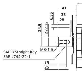
Model Code Option 'K' Shaft
