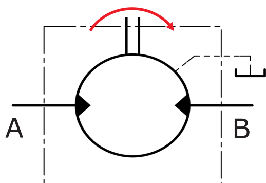
Standard motor
